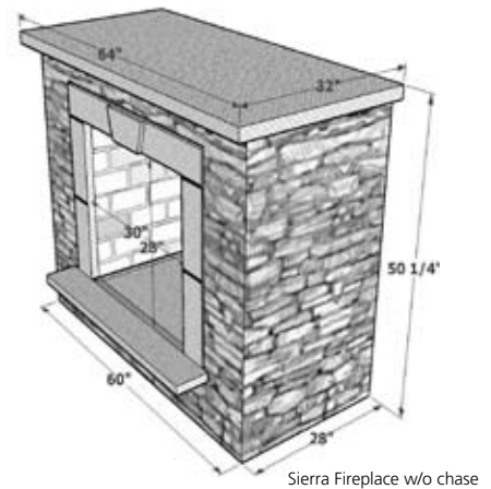
Sierra Fireplace w/o chase
